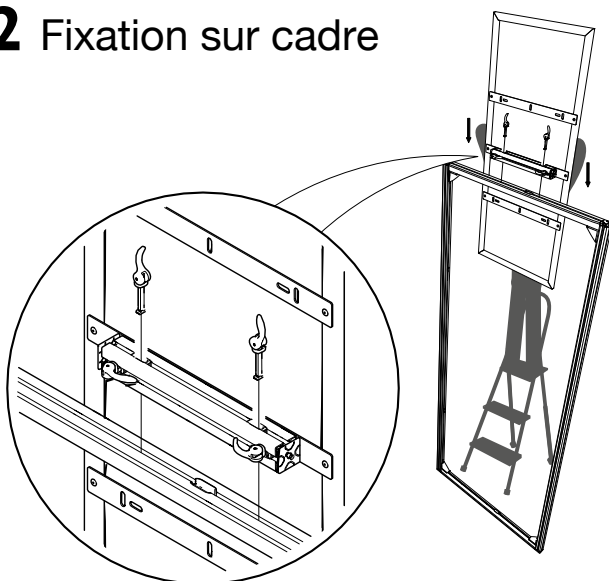
Format rectangulaire vertical 480x1200 mm
